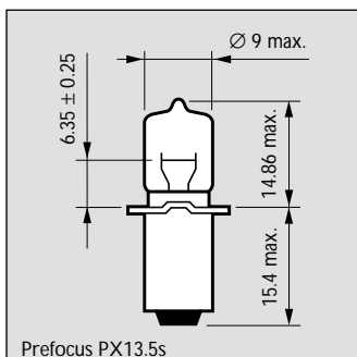
Prefocus PX13.5s
